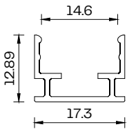
Profile Cross Section Curved Profile Scale 1:1
